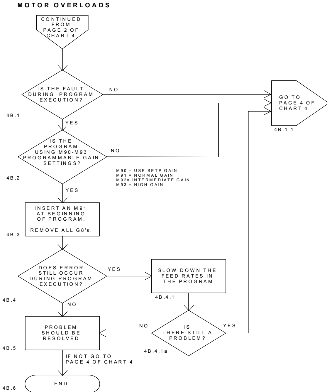
Figure 16-11 Axis Control (Continued)
