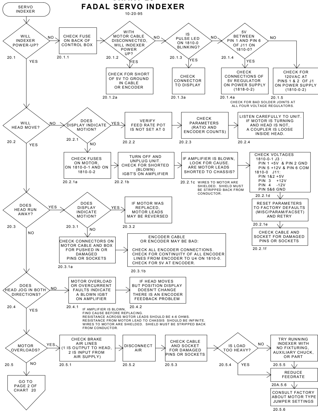
Figure 16-31 Servo Indexer
